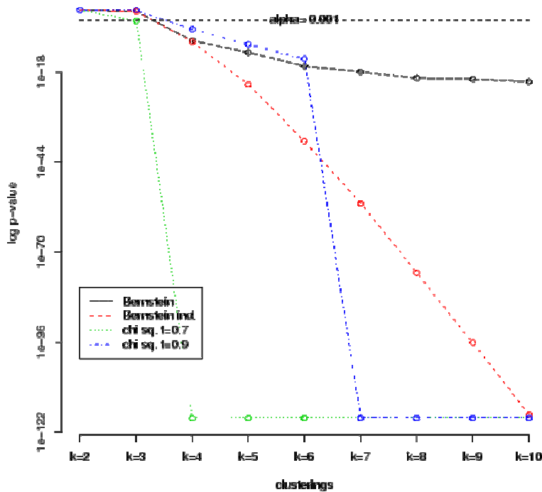
Figure 1: K-means clustering: \log p -values computed for \chi^2 -based and Bernstein -based statistical tests. Ordinate: \log p -value; abscissa: number of clusters sorted according the computed stability indices.
